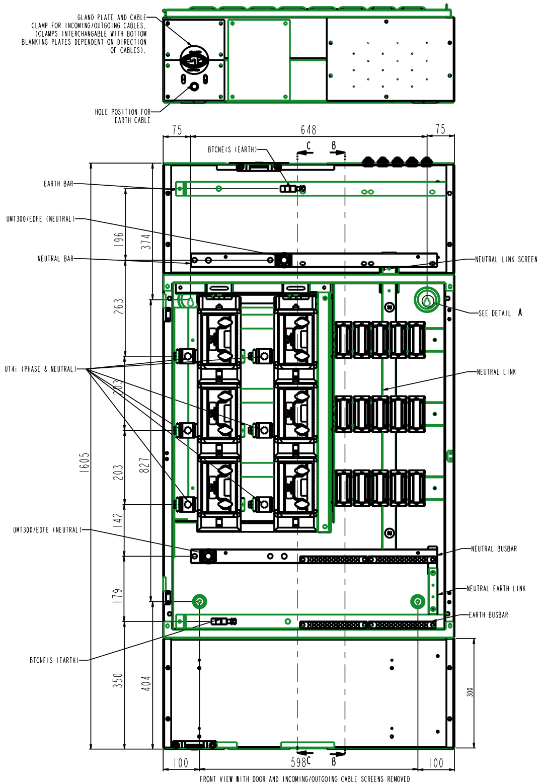
FRONT VIEW WITH DOOR AND INCOMING/OUTGOING CABLE SCREENS REMOVED
