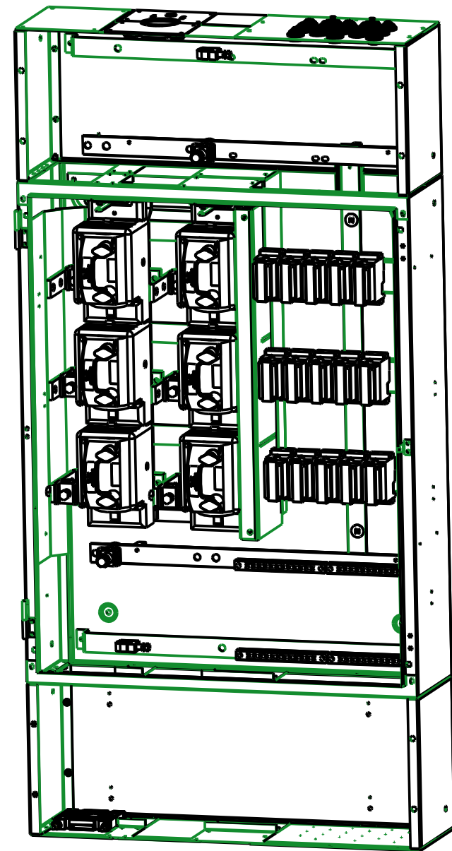
ISOMETRIC FRONT VIEW WITH DOOR REMOVED
