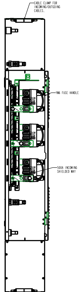
SECTION C-C SHOWING 500A INCOMING SHIELDED FUSEWAY
