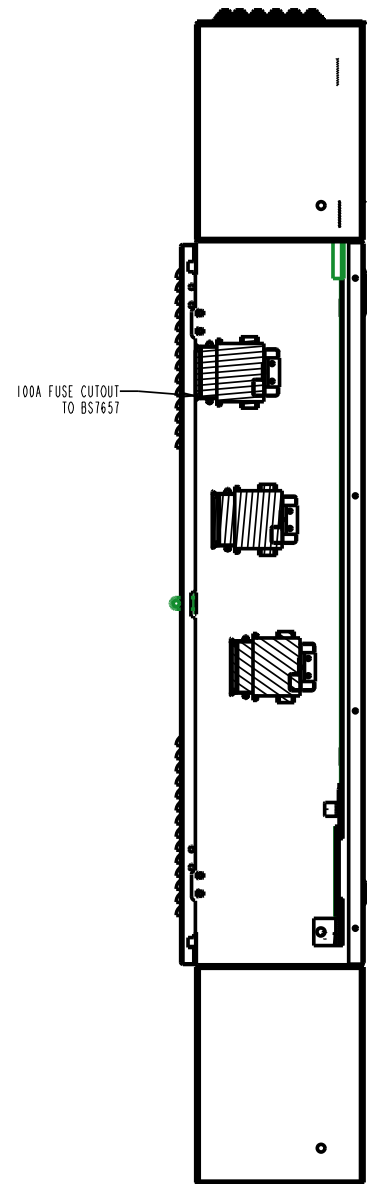
SECTION B-B SHOWING 100A FUSE CUTOUTS
